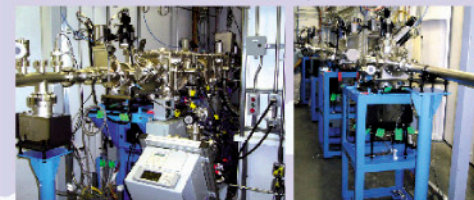
VESPERS Beamline
